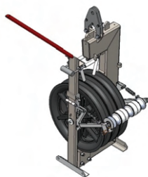
With pressure roller for aluminum and polyamide groove liner OPTIONAL: with carbon brushes
